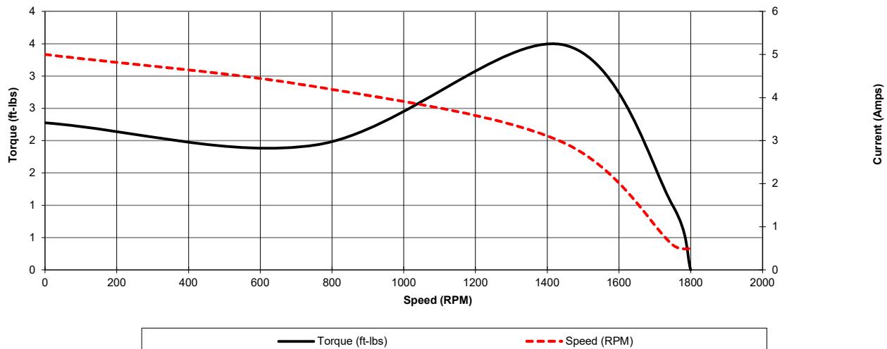
443T - 484T Dual Voltage DOL & 1 leads WYE Connection
